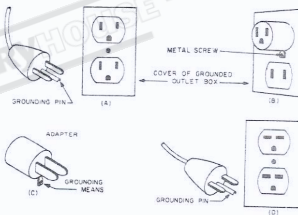
FIGURE 1 GROUNDING METHODS
